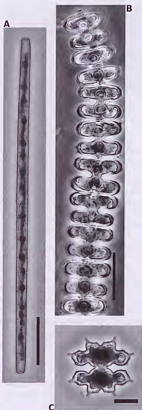
Figure 2. A. Haplotaenium minutum var. elongatum , 200 \times mag. Brightfield. Scale Bar = 40 \mu m; B. Sphaerosoma aubertianum var. indicum , 400 \times mag. Phase contrast. Scale Bar = 20 \mu m; C. Euastrum planctonicum , faceview, 400 \times mag. Brightfield. Scale Bar = 10 \mu m.
